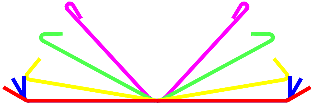
FLOWER DIAGRAM - 45 MM STRIP, 240 MM SET WIDTH
